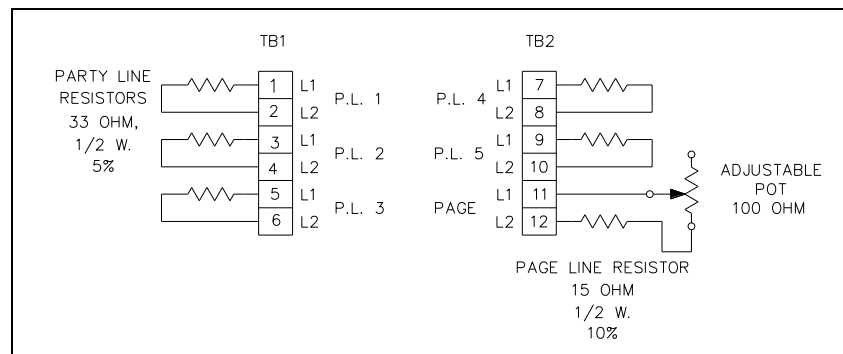
Figure 1. Line balance assembly terminal block connections
